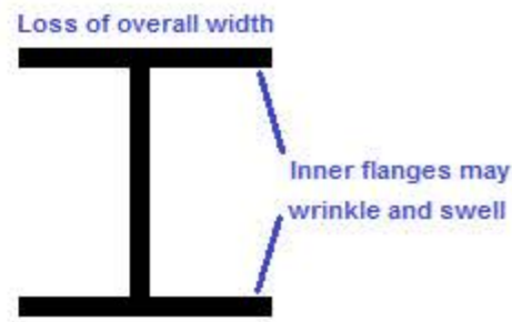
Beam - "Crawl"
