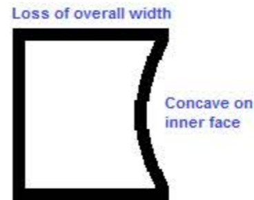
Square Tube
