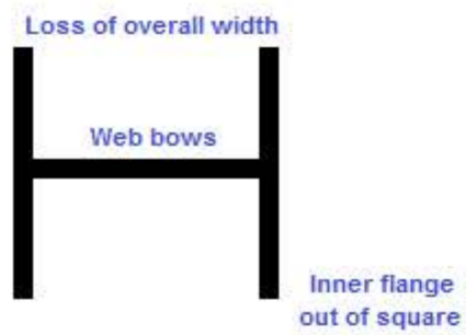
Beam - "Hardway"
